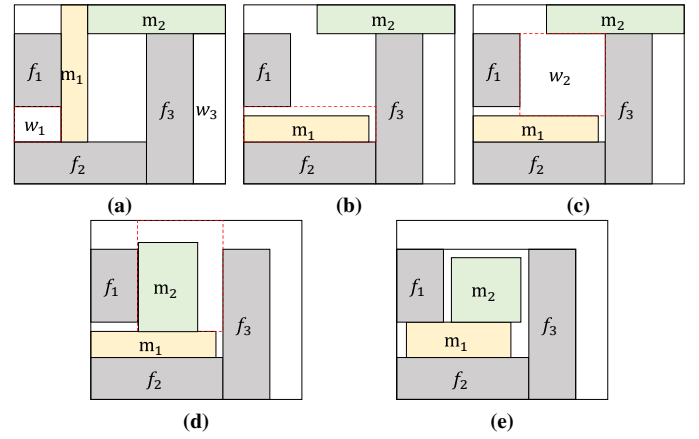
Fig. 3: Relocate modules adjacent to whitespace.
