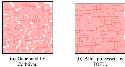
Fig. 5: Floorplans of n300.
